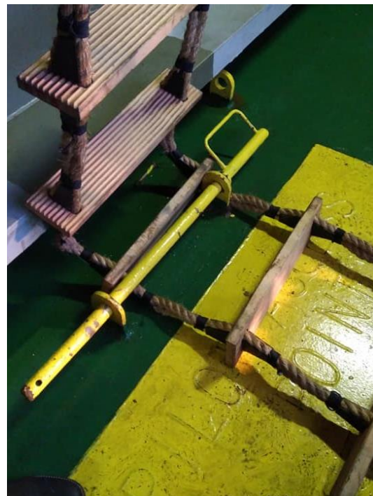
Steel Bar: damaging to the chocks and steps of the ladder
