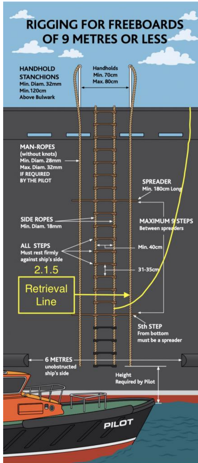
The Steps: Detail of Wheelhouse poster
