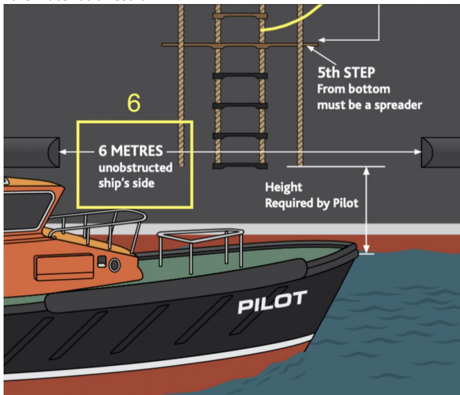
Safe Approach; Detail of Wheelhouse poster
