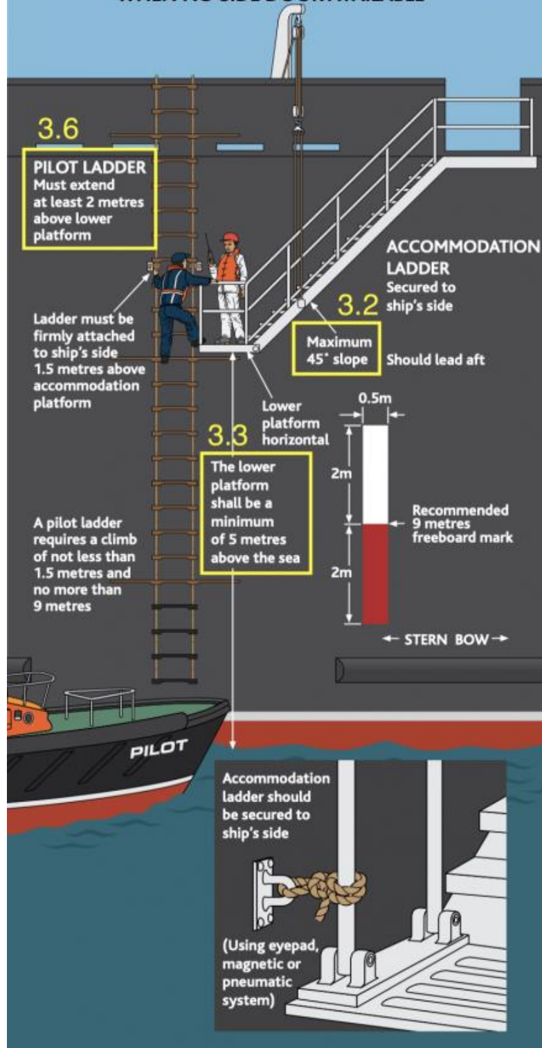
Combination Ladders; Detail of Wheelhouse poster
