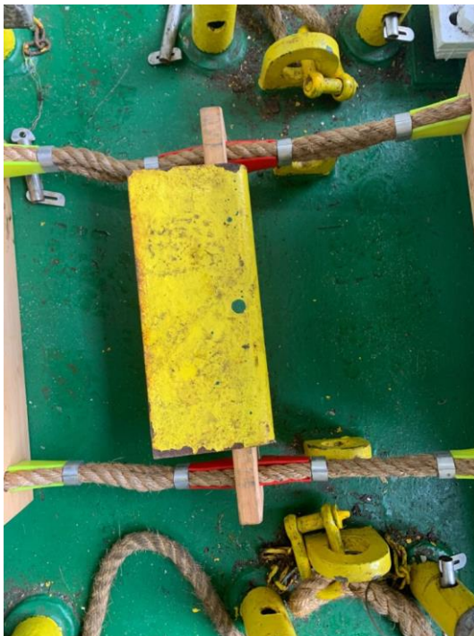
Deck Tongue: all weight rests on the steps
