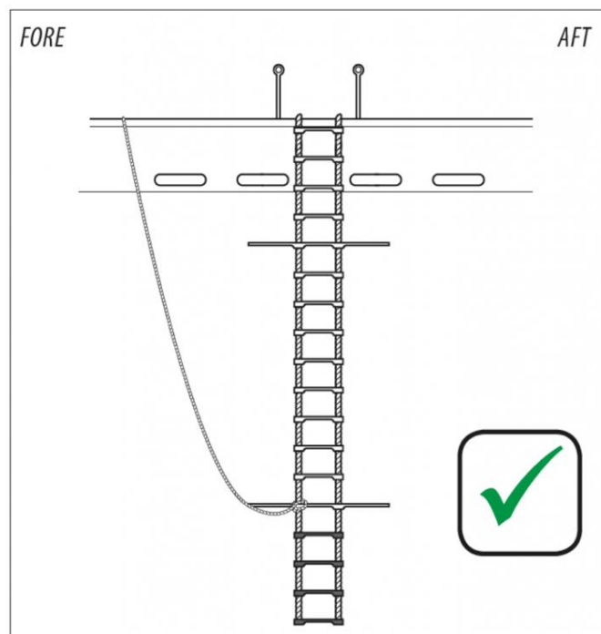
Retrieval line: At or above the spreader, leading forward
