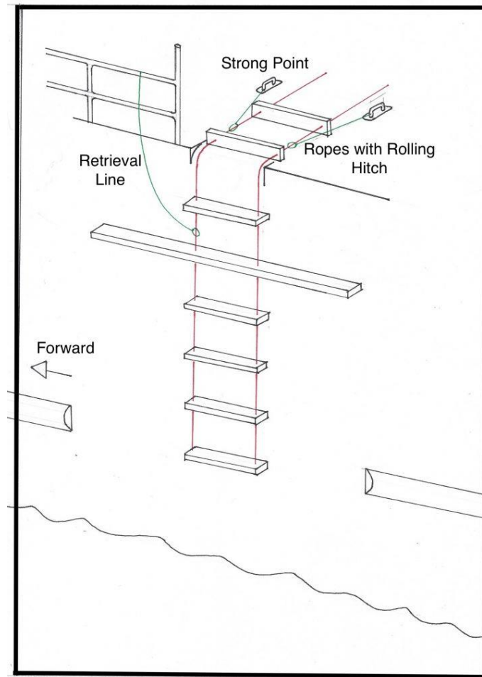
Securing of the Pilot Ladder
