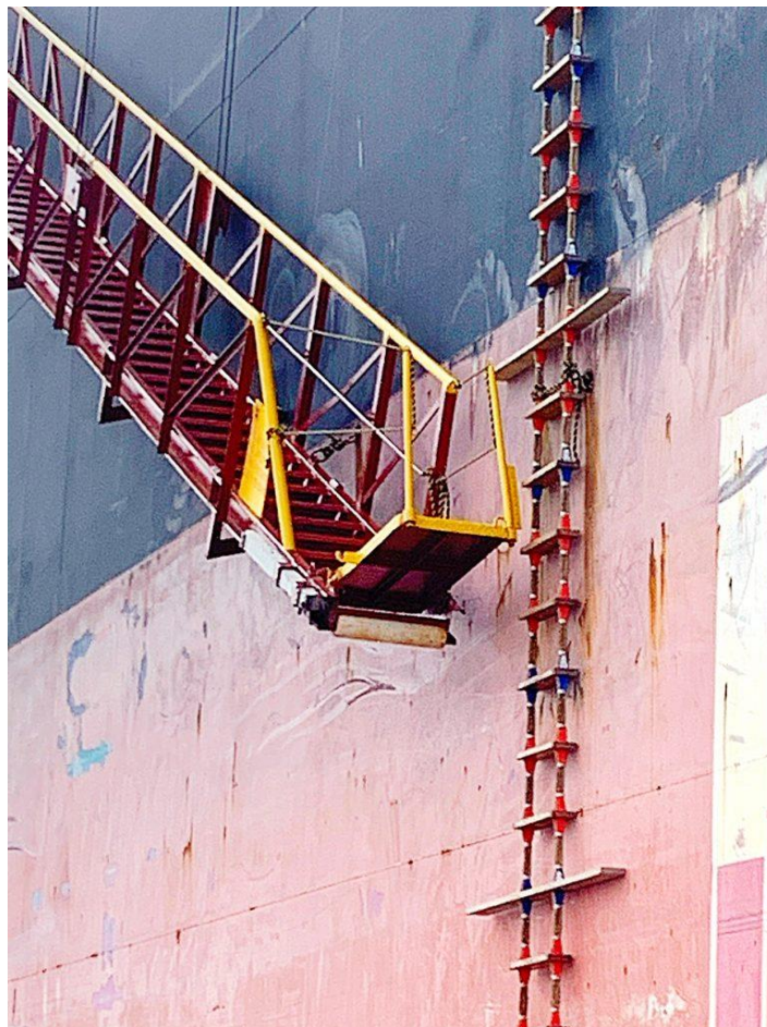
A well secured combination pilot ladder
