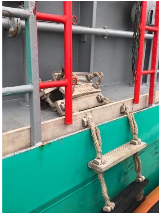
The spreader as a securing device: it is not designed to carry the weight
