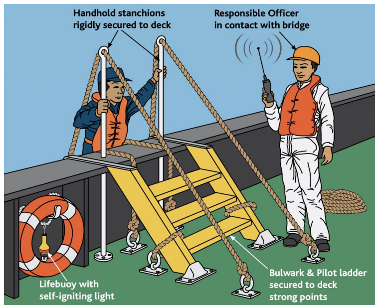
Access to Deck Detail of Wheelhouse poster
