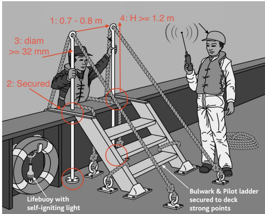
Main features of the handhold stanchions (Detail of Wheelhouse poster)
