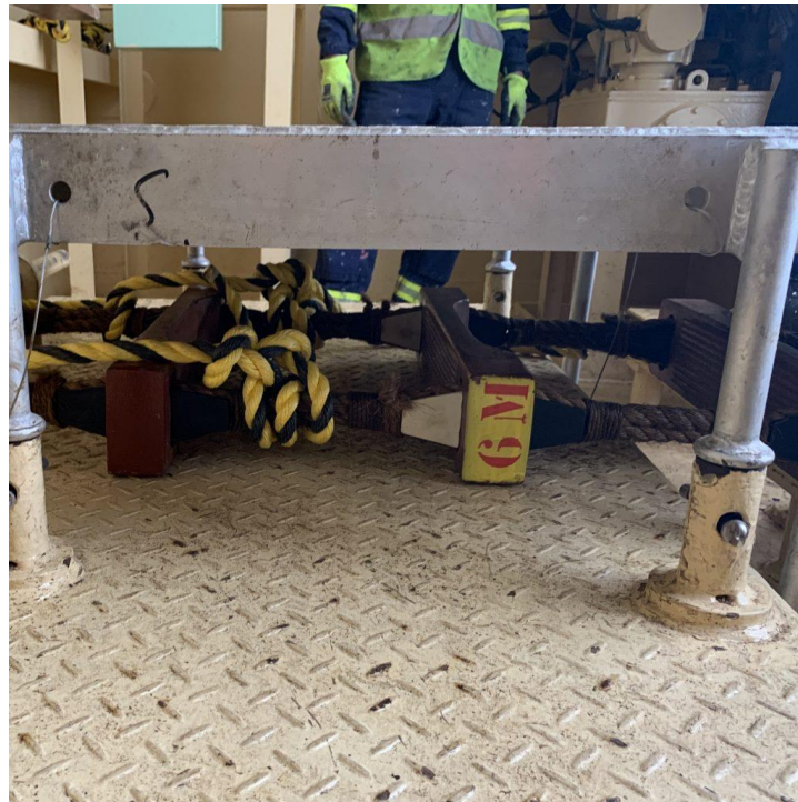
Pilot ladder from a winch, secured by rolling hitch knots.
