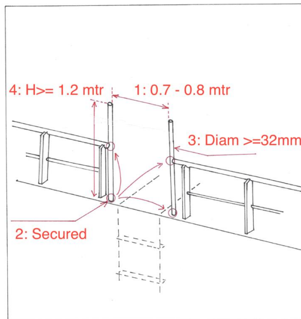
Main features of the handholds
