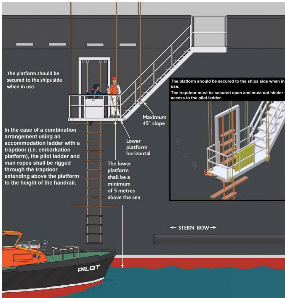
Trapdoor Arrangements: Detail of proposed change to the wheelhouse poster
