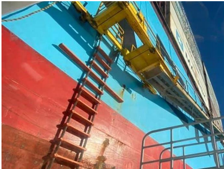
A non-compliant trapdoor arrangement: Pic: Marinelog article
