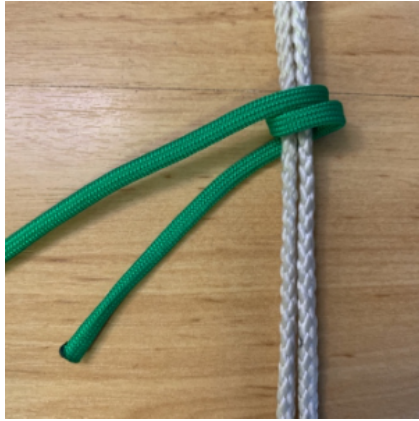
rolling hitch 1
