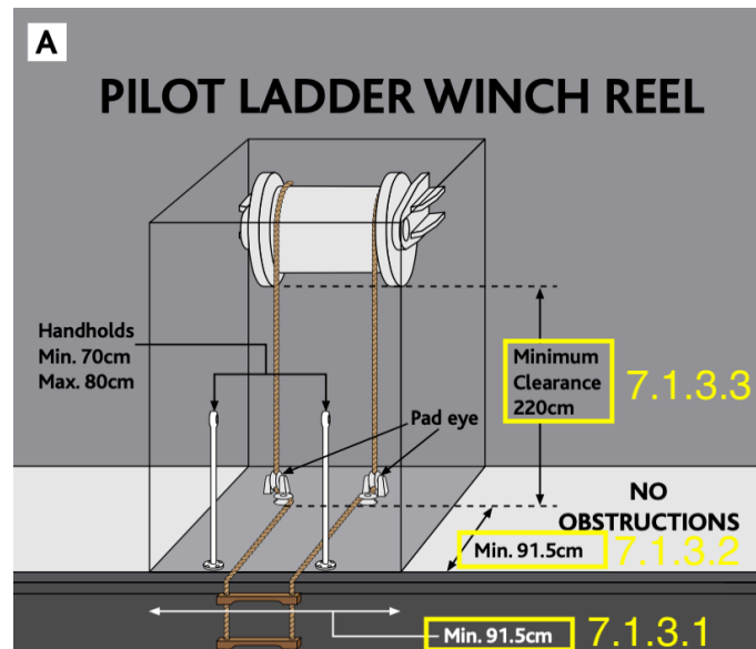
Winch Reel Arrangements; Source: Wheelhouse Poster
